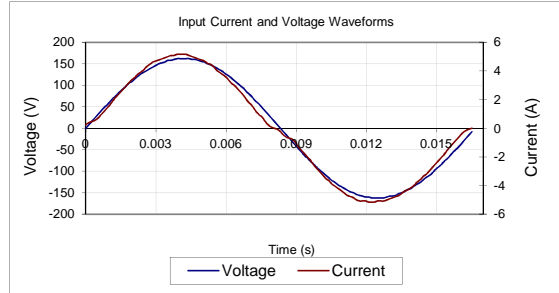
Input AC Current Waveform (THD = 7.17%, 50% Load)
